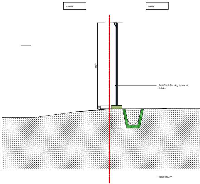
FENCING SECTION
